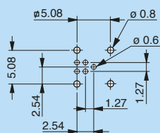
P10 - EPG.00.305
