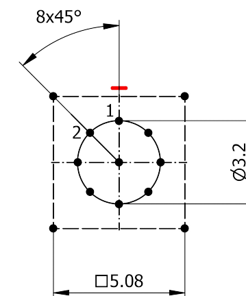
Recommended PCB Layout PCB Top View
