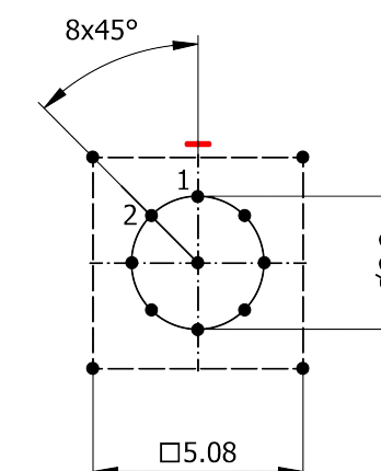
Recommended PCB Layout PCB Top View
