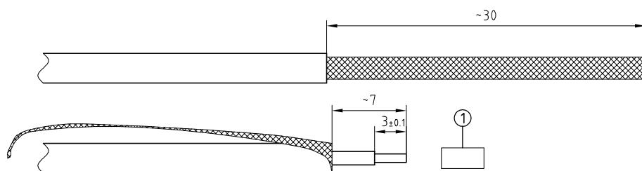
Stripping dimensions
