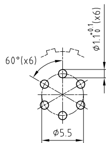
PCB drilling pattern
