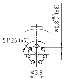
PCB drilling pattern
