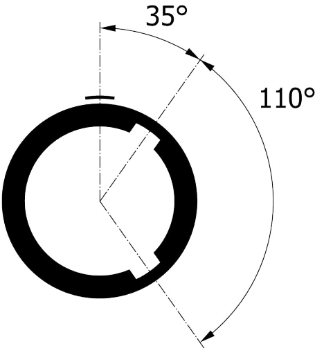
Alignment Key Front View
