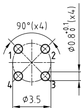
PCB drilling pattern
