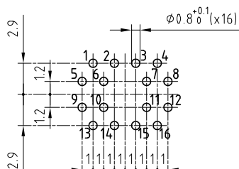
PCB drilling pattern
