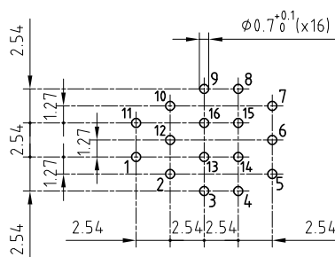
A-A cross-section (PCB drilling pattern)
